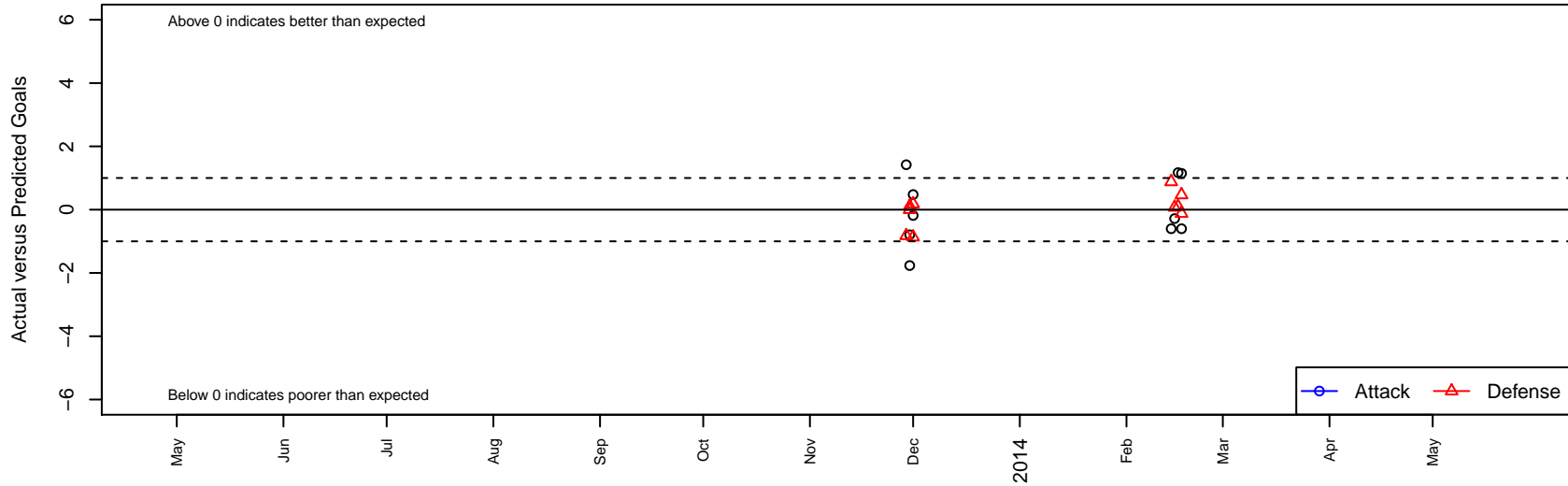
Arizona Arsenal 00 Premier Teal G99 Dots are actual minus expected GF (blue circles) and GA (red triangles). Blue line is smoothed change in attack strength. Red is smoothed change in defense strength.
